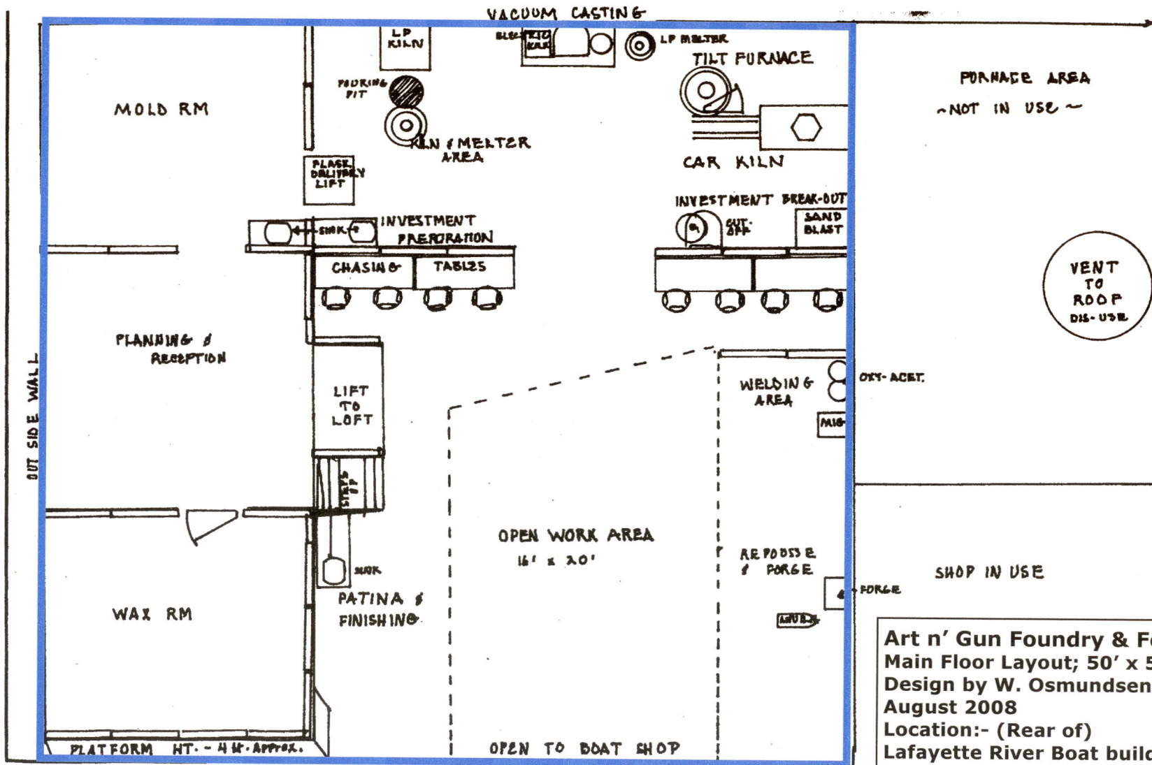
Shop Plan for Bronze Foundry & Forge Overall Area 50 ft. x 50 ft.
